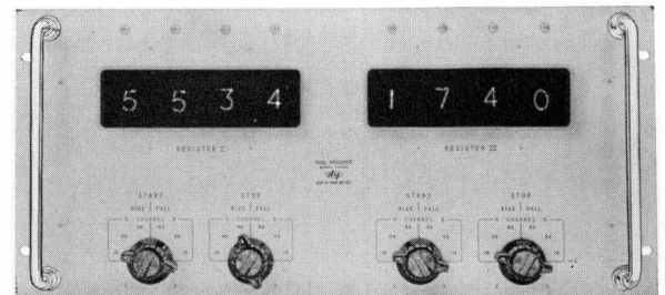
Fig. 3. Dual Register unit selects regions to be evaluated, displays results.
