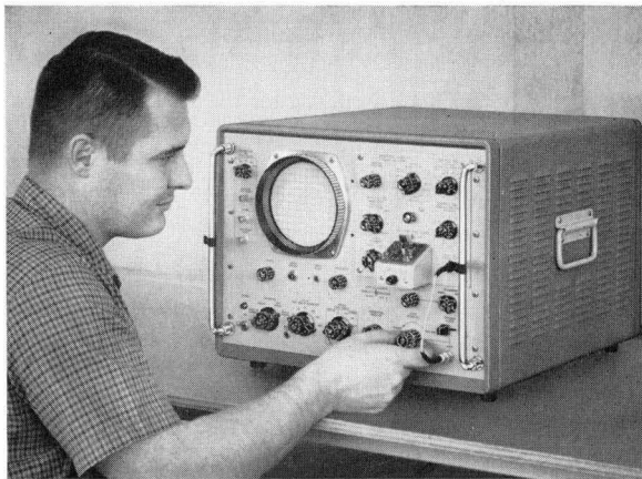
Fig. 1. New -hp- Model 186A Switching Time Tester plug-in operates with -hp- Model 185A or 185B Sampling Oscilloscope to measure rise, fall, switching, and recovery times of fast transistors, diodes, tunnel diodes. Device to be tested simply plugs into test circuit provided on holder. Tester provides fast test pulse and adjustable voltages for operating device.
